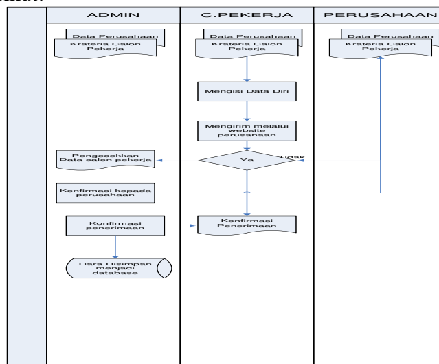
Gambar2. Document Flow
