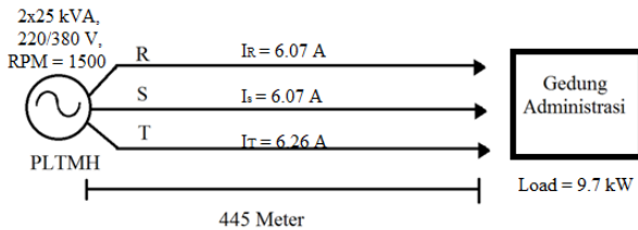
Gambar 4 Single line diagram perencanaan PLTMH
