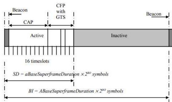
Gambar 2. Superframe Zigbee[4]
