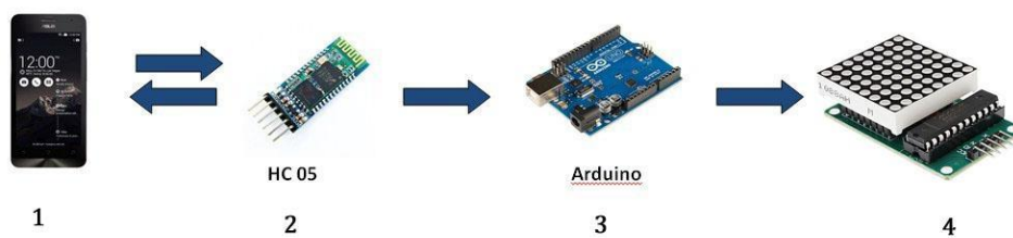
Gambar 1. Diagram Blok
