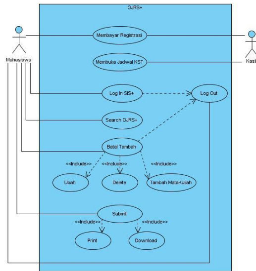
Gambar 10. Use Case Diagram OJRS+
