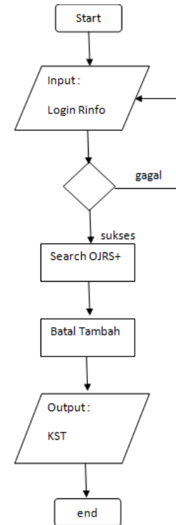
Gambar 11. Flowchart
