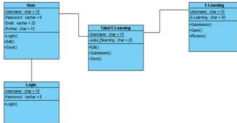
Gambar 3. Class diagram website e-learning
