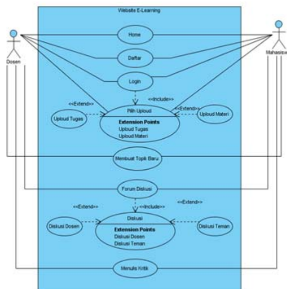
Gambar 2. Use case diagram sistem e-learning
