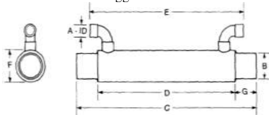
Gambar 6 Double-pipe Liquid Suction Heat Exchanger (LSHX)
