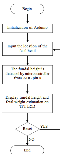
Fig. 2. The Flowchart of the Arduino Program
