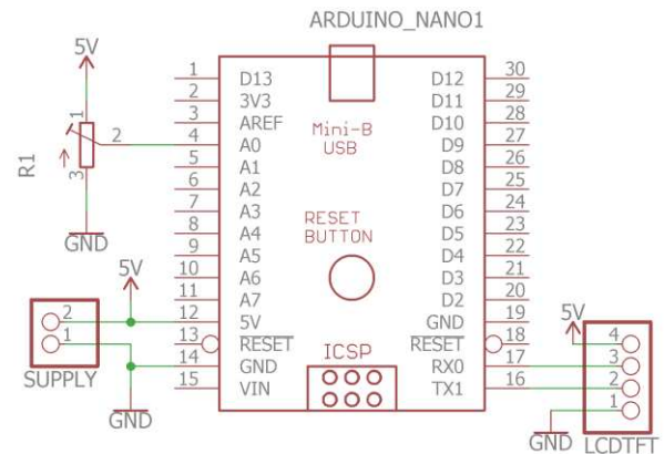
Fig. 3. Height detector circuit
