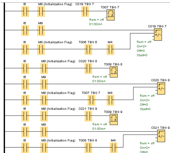
Fig. 11. Ladder timer circuit 7 through 9
