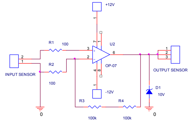
Fig. 6. Thermocouple analog signal conditioner circuit
