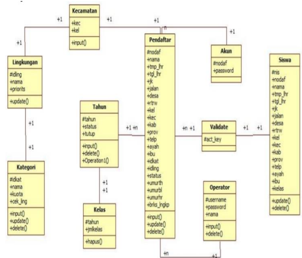
Fig. 4. Class Diagram
