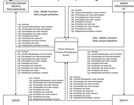
Gambar 3. Context Diagram
