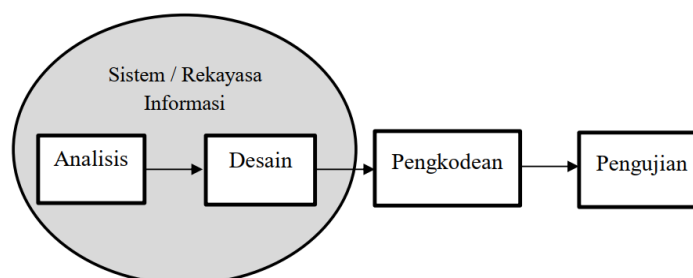
Gambar 2. Model Waterfall
