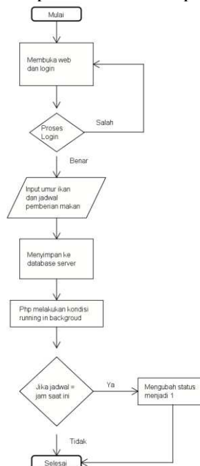
Gambar 5. Flowchart website
