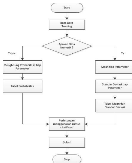
Gambar 2. Flowchart naïve bayes
