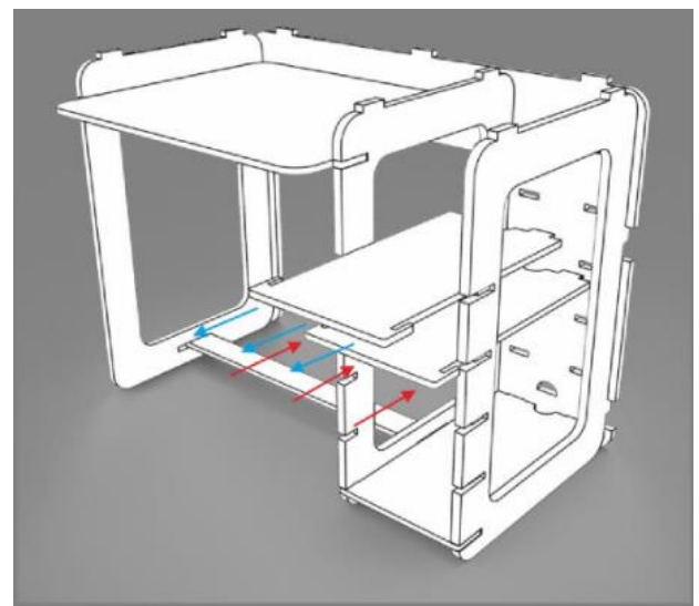
Gambar 10. Possible Slotting Joint type for shelving panel
