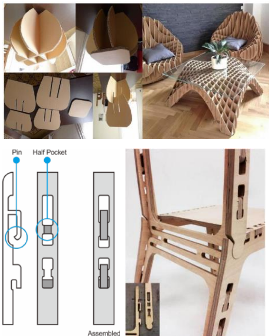
Gambar 3. Slotting Joint
