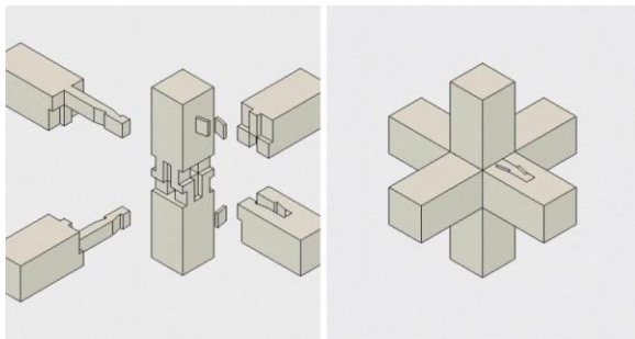
Gambar 2. Joint interlocking system tradisional Jepang (sumber : http:// www.tylco.com )
