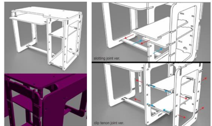
Gambar 13. Reconfigurable Home PC Desk with Clip Tenon joint Interlocking System
