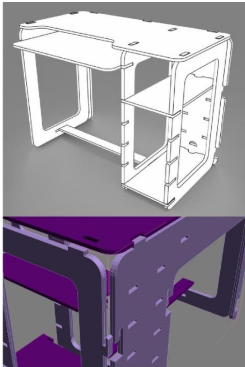
Gambar 9. Reconfigurable Home PC Desk with Slotting joint Interlocking System
