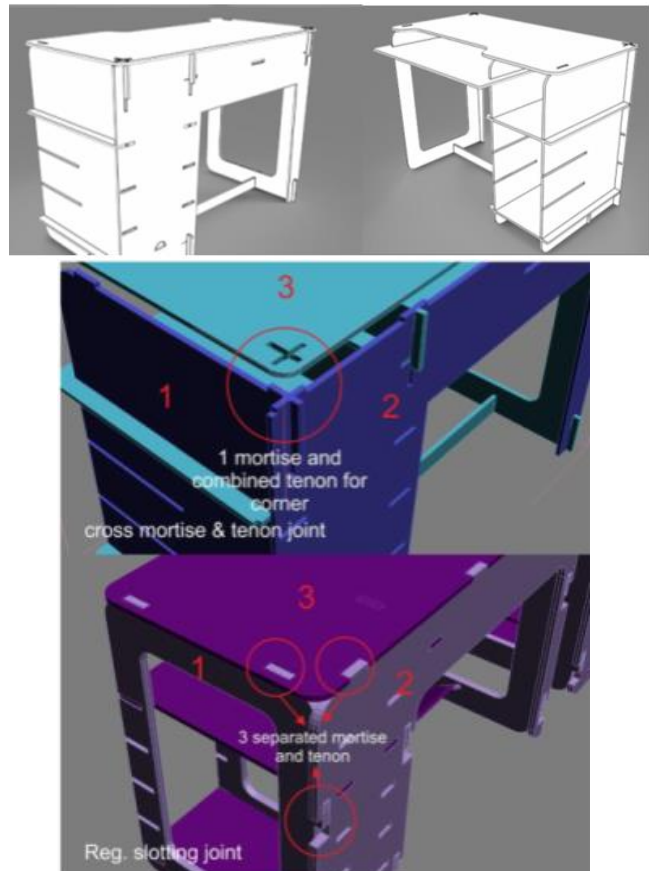
Gambar 16. Reconfigurable Home PC Desk with cross mortise joint Interlocking System
