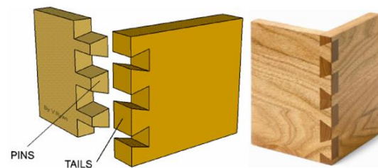
Gambar 6. Hammer joint
