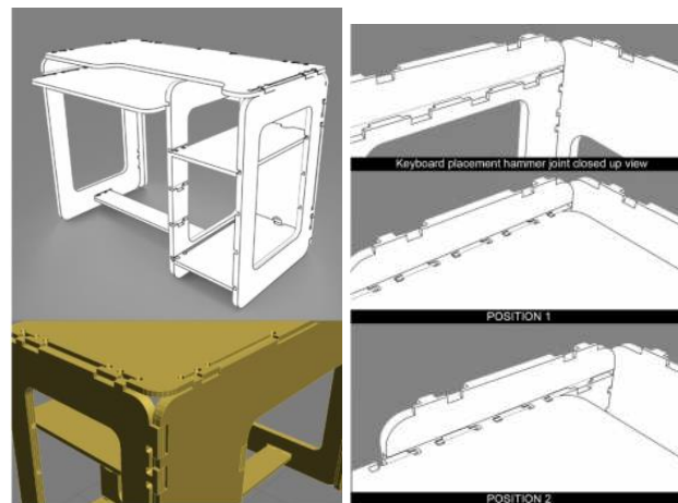
Gambar 15. Reconfigurable Home hammer joint Interlocking System
