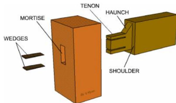
Gambar 5. Traditional Japan Wedged mortise & tenon joint
