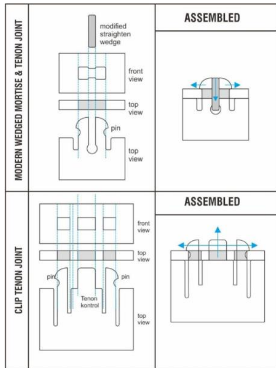
Gambar 14. clip tenon joint vs modern wedged mortise & tenon joint
