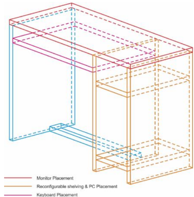
Gambar 8. Frame Base Template Design
