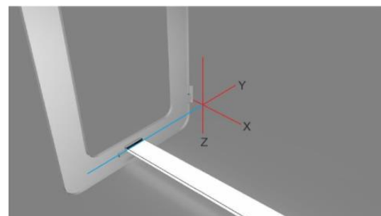
Gambar 11. slotting joint local stability
