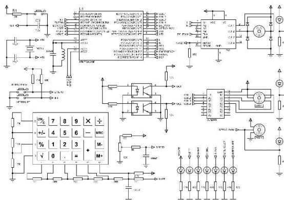
Gambar 9. Wiring diagram Proteus pengendalian motor
