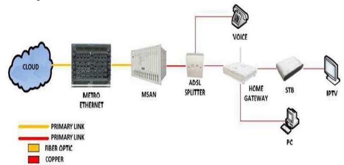
Gambar 2. Topologi MSAN [2]
