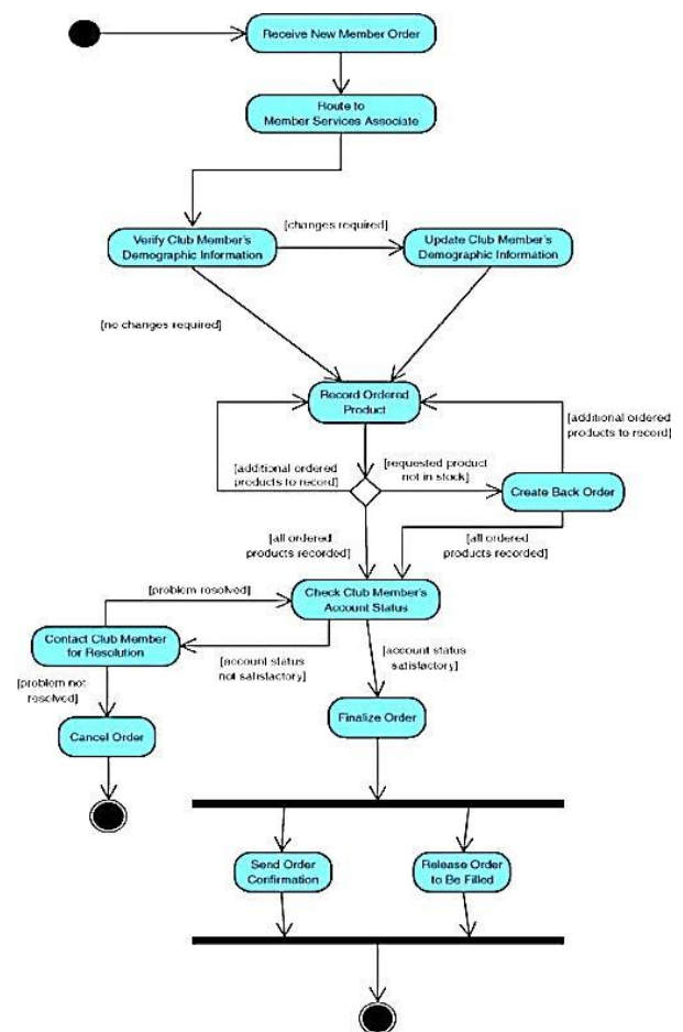
Gambar 4. Activity Diagram
