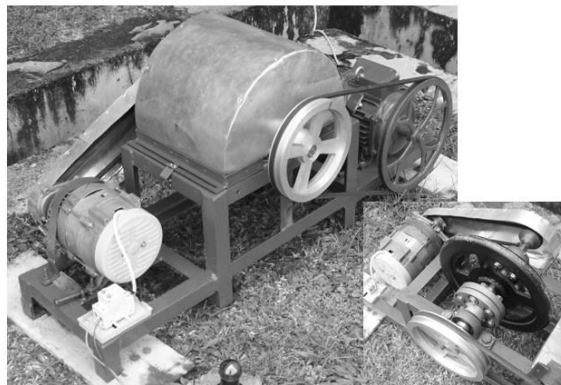
Gambar 6. Mekanisme Model FESS
