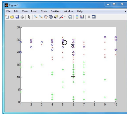
Gambar 4 Plot Clustering
