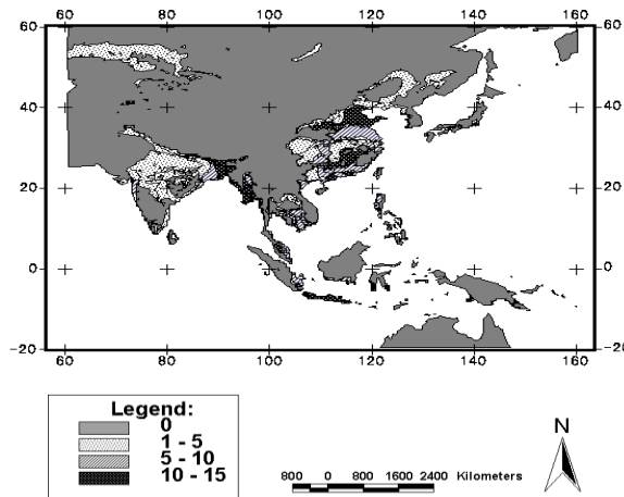
Figure 6. Changes of annual E_a (%) due to land cover changes.
