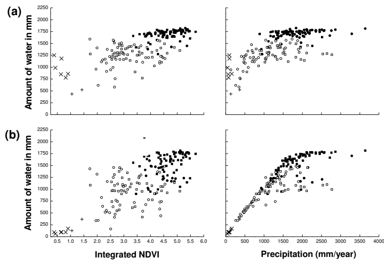
Figure 5. Scatter plots of annual (a) E_0 and (b) E_a versus integrated NDVI and mean annual precipitation of tropical rain forest (■), tropical seasonal forest (●), cropland (○), rice paddy (□), semi desert (+), and bare desert (×).
