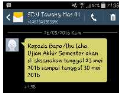
Gambar 6. Output SMS 2
