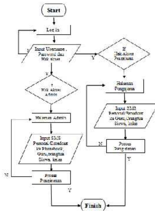
Gambar 1. Proses sms broadcast
