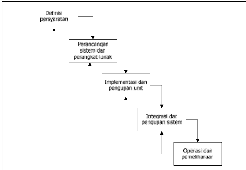
Gambar 2. Metode Waterfall [10]
