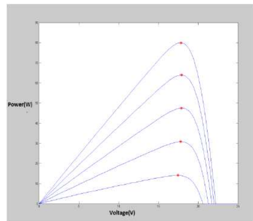
Figure 3(b): P-V characteristics corresponding to I-V characteristics (red dot shows maximum power point (MPP) [7]
