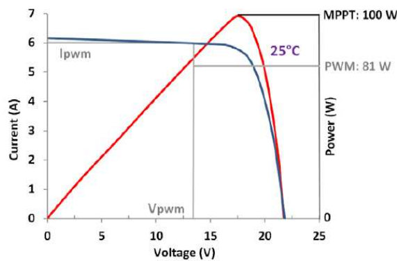
Figure 2: Current Vs Voltage curve for PWM [5]
