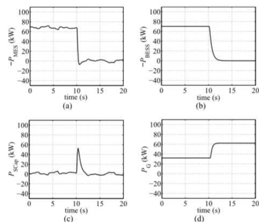
Fig. 7: Case B: Droop-control-based responses to wind fluctuation and fast charging when SOC of the battery is lower than the scheduled: (a) Multilevel energy storage system (MES) charging power from the DC bus, (b) Battery charging power from the DC bus, (c) Supercapacitor discharging power to the DC bus, (d) Grid power to the DC bus [1]
