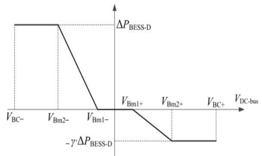
Fig. 5: Droop control of the BESS to mitigate the power deviations of DC microgrid in higher than the scheduled SOC of the BESS [1]
