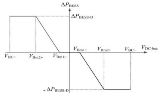
Fig. 3: The Droop control of a BESS power electronic converter to mitigate power deviations of DC microgrid in normal condition of the BESS [1]
