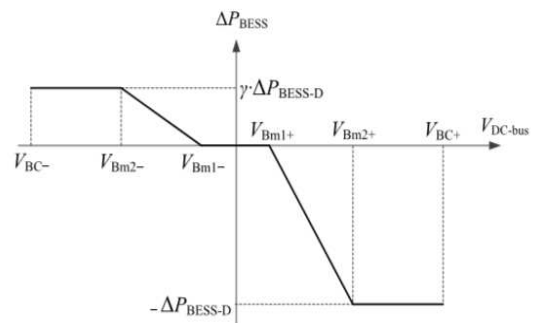
Fig. 4: Droop control of BESS power electronic converter to mitigate the power deviations of DC microgrid is lower than the schedules SOC of the BESS [1]
