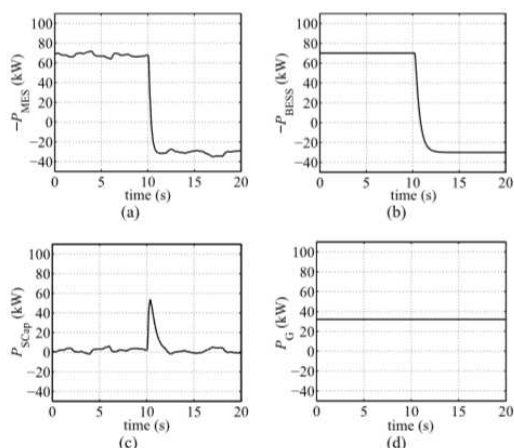
Fig. 6: Case A: Droop-control-based responses to wind fluctuation and fast charging when SOC of the battery is as scheduled: (a) Multilevel energy storage system (MES) charging power from the DC bus, (b) Battery charging power from the DC bus, (c) Supercapacitor discharging power to the DC bus, (d) Grid power to the DC bus [1]
