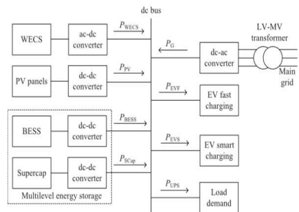
Fig. 1: Layout of a DC microgrid [1]
