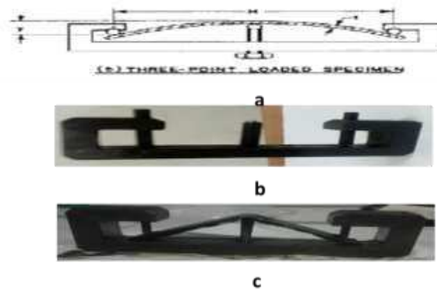
Figure 1. Holder shape and installation of test specimens.
