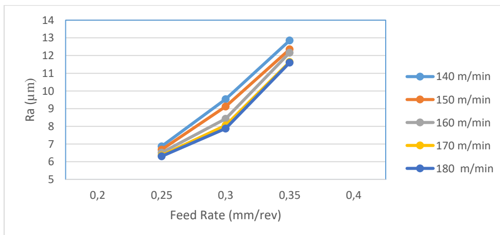
Figure 6. Graphic Feed Rate Vs. Surface Roughness Source
