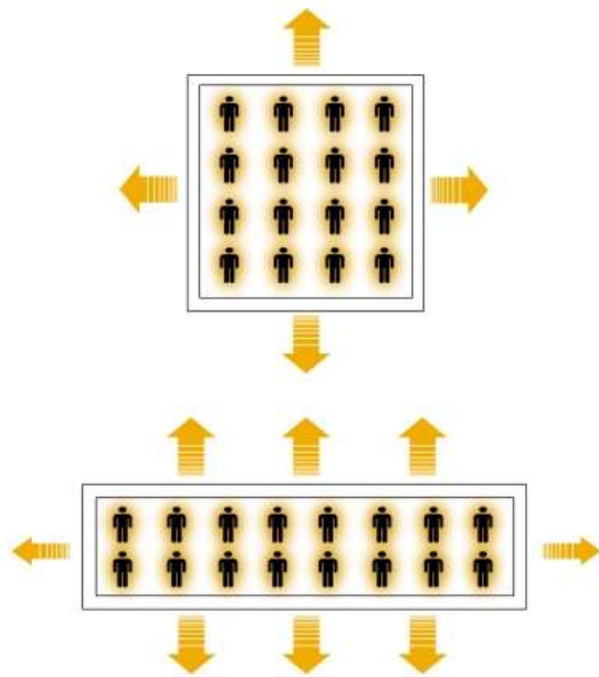
Figure 6. Thinner buildings lose more of their internal heat to the outside (Workshop, 2014)
