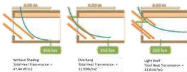
Figure 12. Example of Light Shelf Performance (Suryabrata, 2013)
