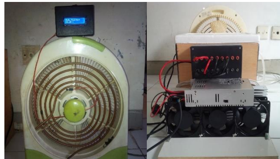
(a) Indoor Sistem Pendingin (b) Outdoor Sistem Pendingin
