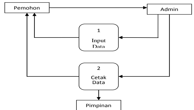
Gambar 6. DFD Level 1
