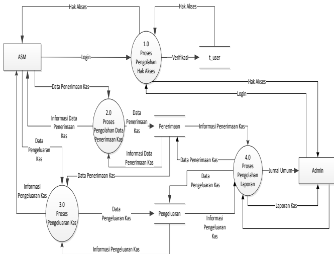
Gambar 6. DFD Level 1
