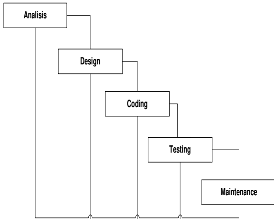
Gambar 1. Model Waterfall
