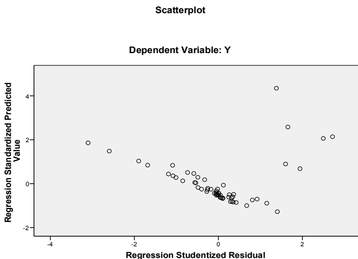
Gambar 4.3. Scatterplot
