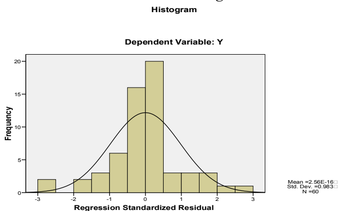
Gambar 4.1. Histogram
