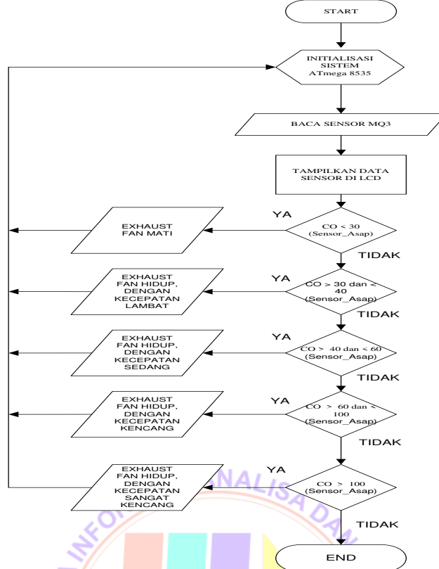
Gambar 1. Flowchat sisten
