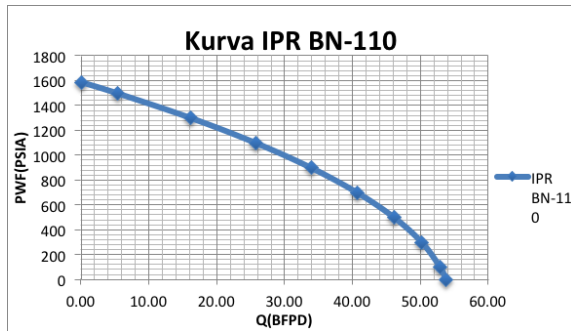
Gambar IV. 7 Kurva Inflow Performance
