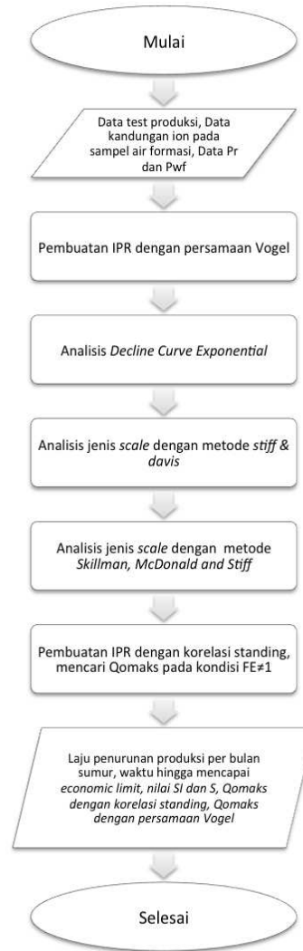
Gambar III. 1 Diagram Alir
