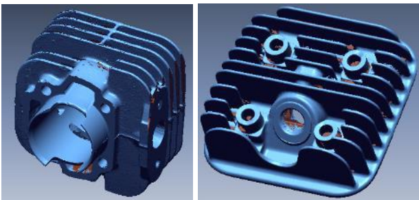
Gambar 6. Polygon mesh
