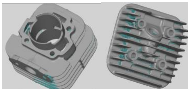
Gambar 4. Data stl blok silinder & Comp.Head
