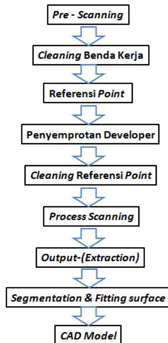
Gambar 2. Flow proses scanning blok silinder & comp. Head
