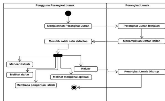
Gambar 4. Activity Diagram
