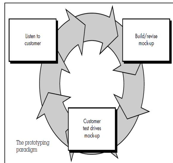
Gambar 1. Metode Prototyping
