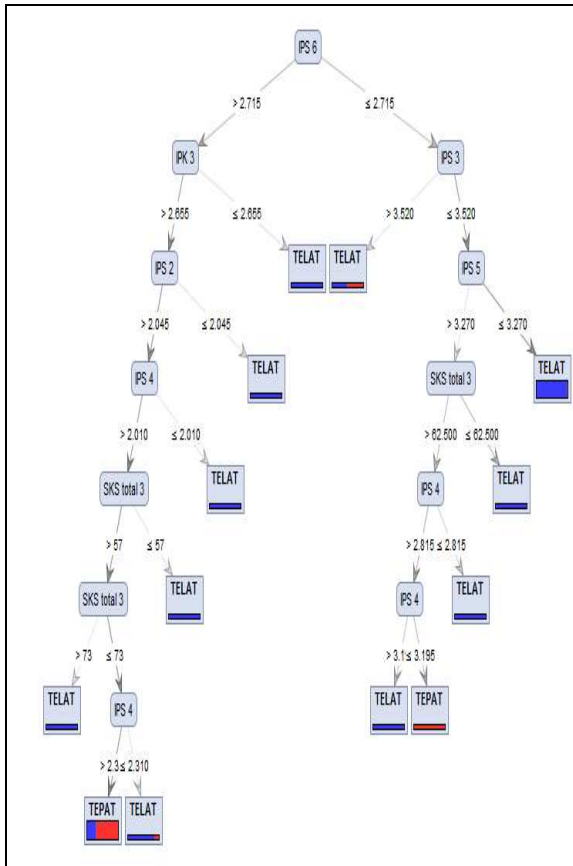
Gambar 1. Pohon keputusan berdasarkan gain ratio
