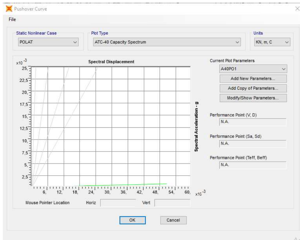
Gambar 3. Pushover Curve
