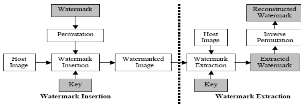
Gambar 1. Block Diagram system watermarking
