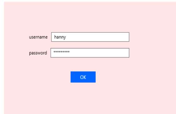
Gambar 8. Form Login
