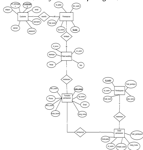
Gambar 4. ERD (Entity Relationship Diagram)
