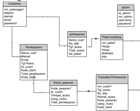
Gambar 5. LRS (Logical Relational Structure)
