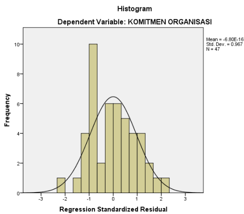
Gambar 3. Histogram
