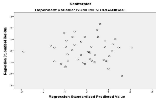
Gambar 2. Scatterplot
