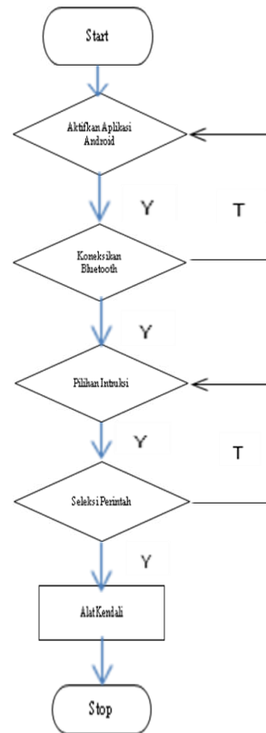
Gambar 9. Flowchart
