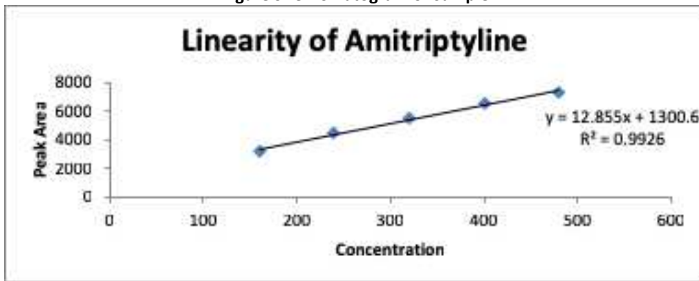
Figure 10: Calibration graph of Amitriptyline
