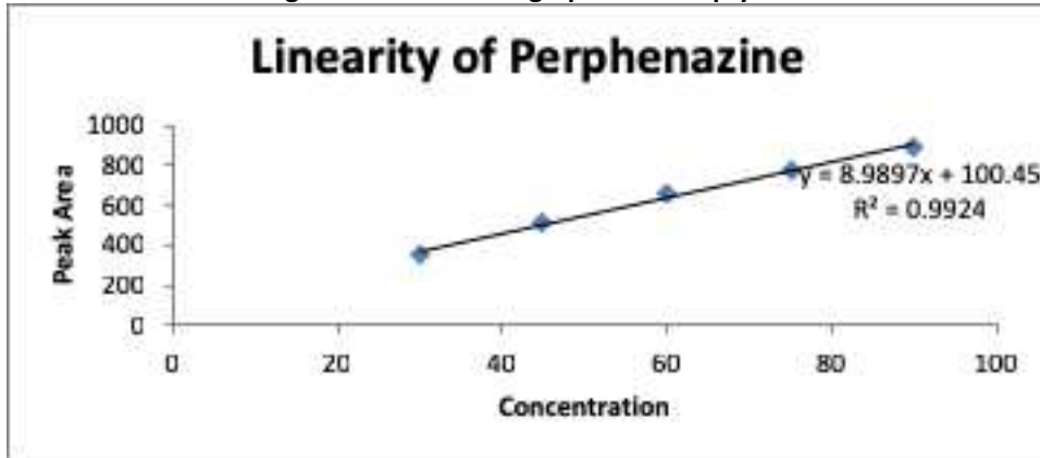
Figure 11: Calibration graph of Perphenazine
