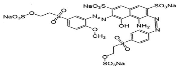
Fig. 1. Structure of Reactive Blue 250.
