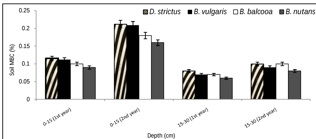
Fig. 2. Variation in soil microbial biomass carbon (MBC) in all study sites with depth and time.
