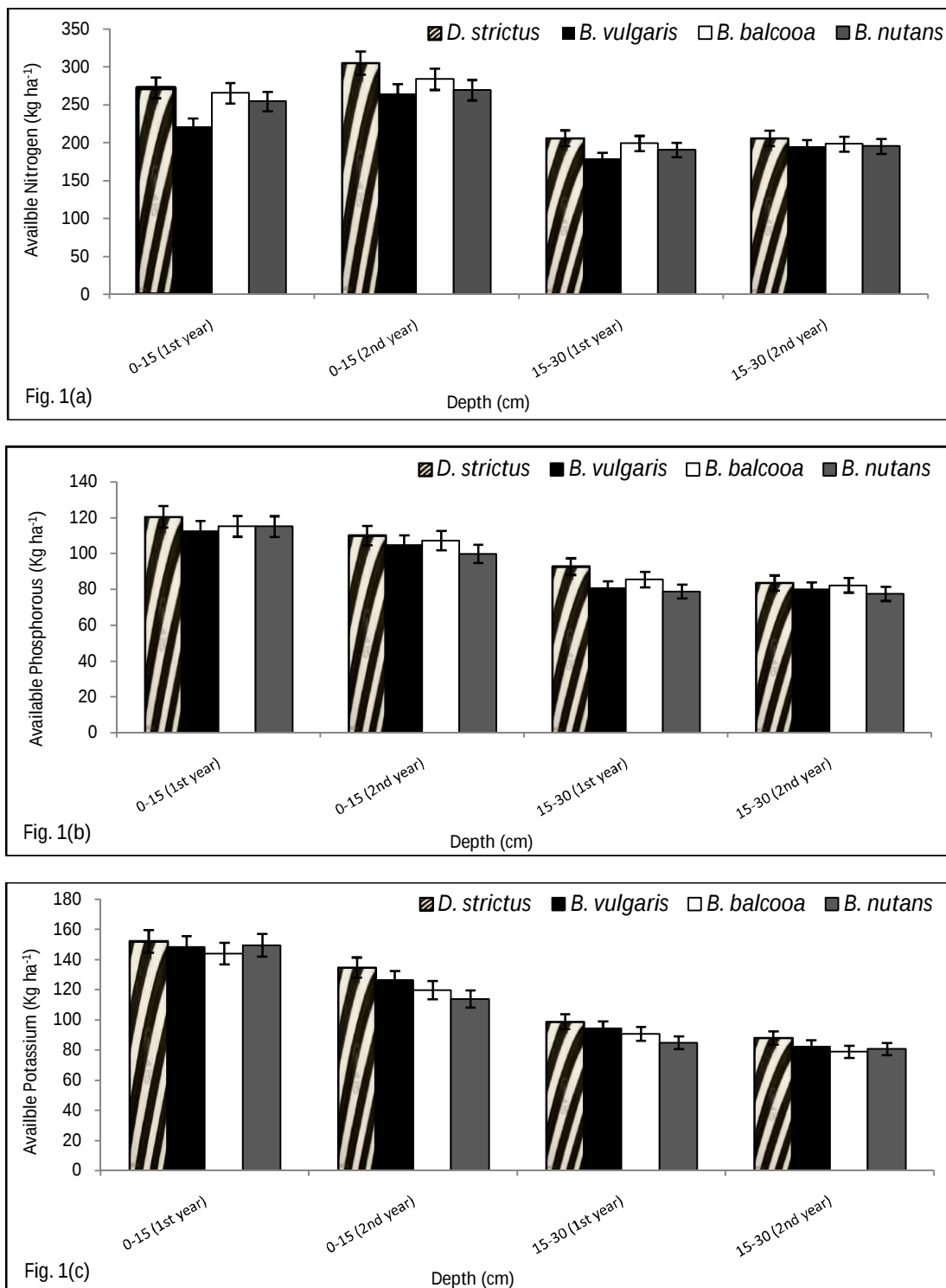
Fig. 1(a,b & c). Change in available soil nitrogen, phosphorous, and potassium in all plantation sites with depth and time.
