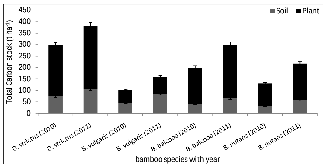
Fig. 4. Comparative soil and plant carbon stocks in all bamboo species with time.
