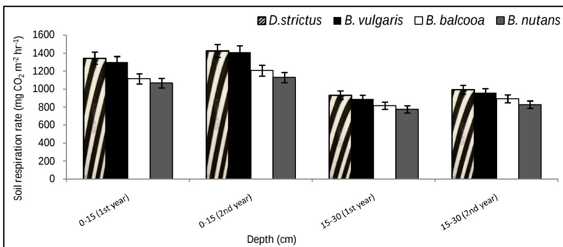
Fig. 3. Variation in soil respiration in all study sites with depth and time.
