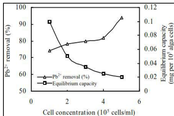
Fig. 2. The effect of spirulina concentration on Pb 2+ Removal and maximum adsorption capacity (Pb 2+ : 30mg/L, temperature: 25°C, agitation speed: 166 rpm) (Adopted from Chen Hang et al. ).
