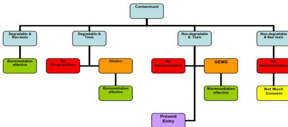
Fig. 1. Bioremediation: Influence of contaminant type.
