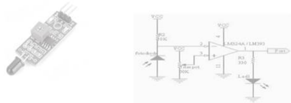
Gambar 2 (a) Modul Flame Sensor (b)Rangkaian Sensor Infra Red
