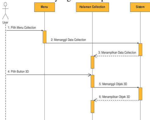
Gambar 11. Sequence Diagram Menu Collection
