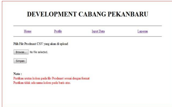
Gambar 3.6 Upload Prodmast
