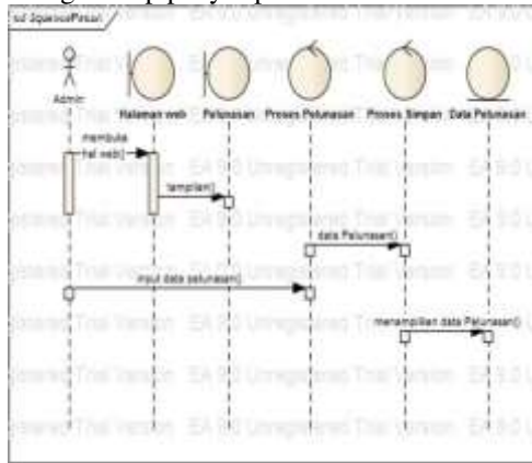
Gambar 12. Sequence Diagram Pelunasan
